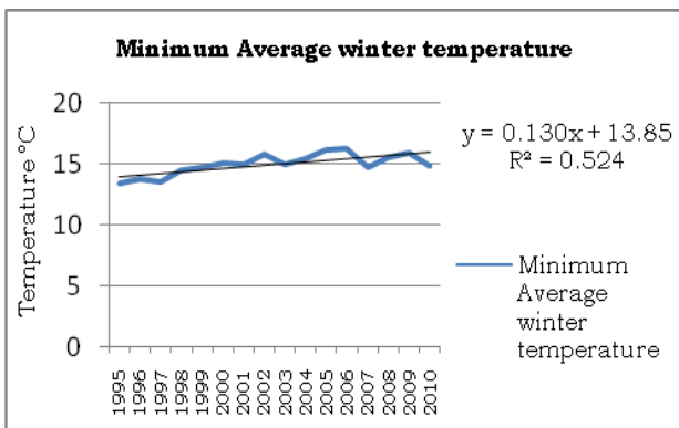
Fig. 4. Trend of minimum average winter temperature
