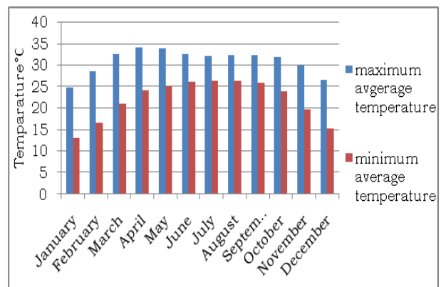
Fig. 1. Monthly average maximum minimum temperature (°C) during period 1995-2010.
