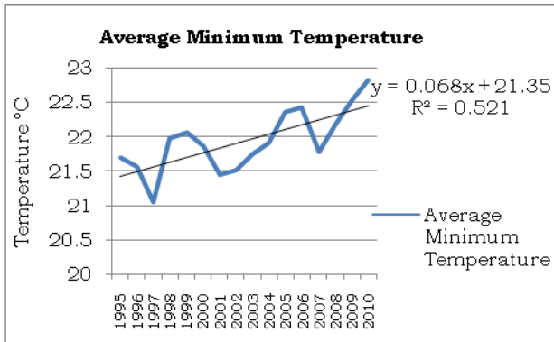
Fig. 3. Trend of monthly minimum temperature data of 1995-2010 periods.
