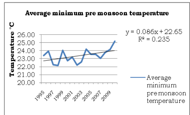
Fig. 6. Trend of monthly minimum temperature data of 1995-2010 in Pre- monsoon periods.
