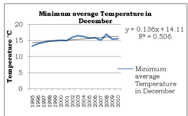
Fig. 7. Trend of monthly minimum temperature data of 1995-2010 in the month of December.
