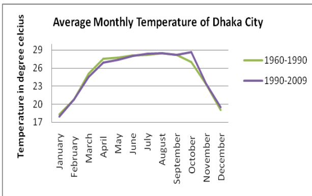
Fig. 2. Change in monthly mean temperature of Dhaka
